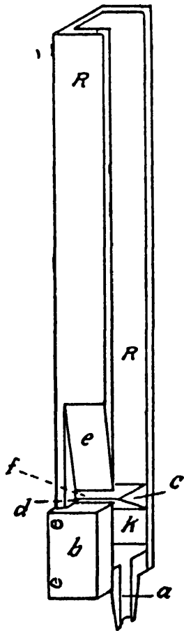
FIGURE 84. Wooden flue-pipe. R body, a foot, b cap, c block, d flue, e toplip, f mouth, k wind way.
